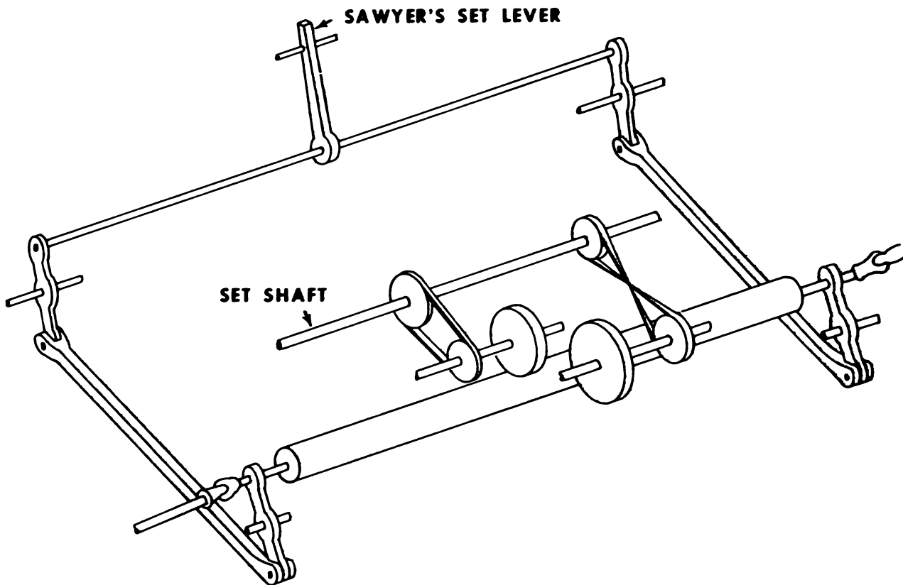
Figure 8-21. Drum-actuated setworks.
